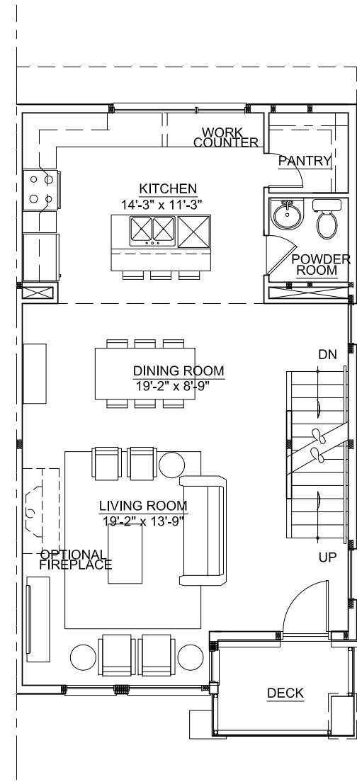
SECOND FLOOR PLAN 675 G.S.F. 0 1 2 4 6 8 FT.
