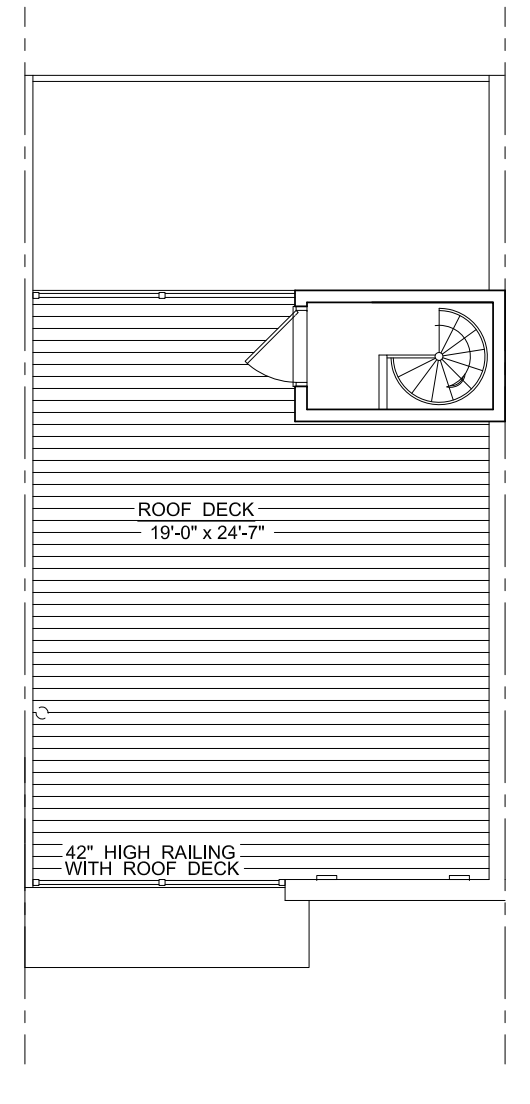
ROOF PLAN 47 G.S.F. 0 1 2 4 6 8 FT.
