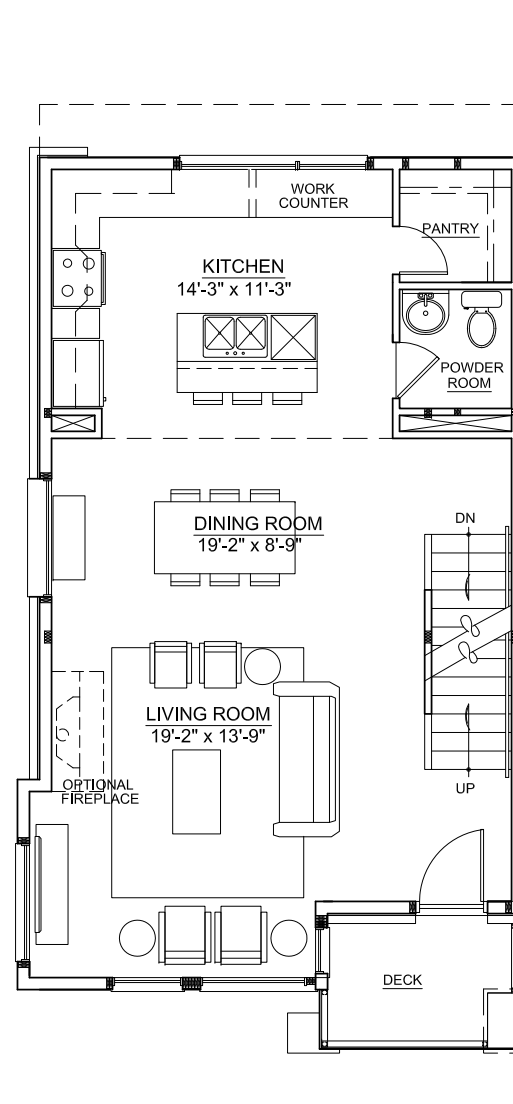
SECOND FLOOR PLAN 691 G.S.F. 0 1 2 4 6 8 FT.
