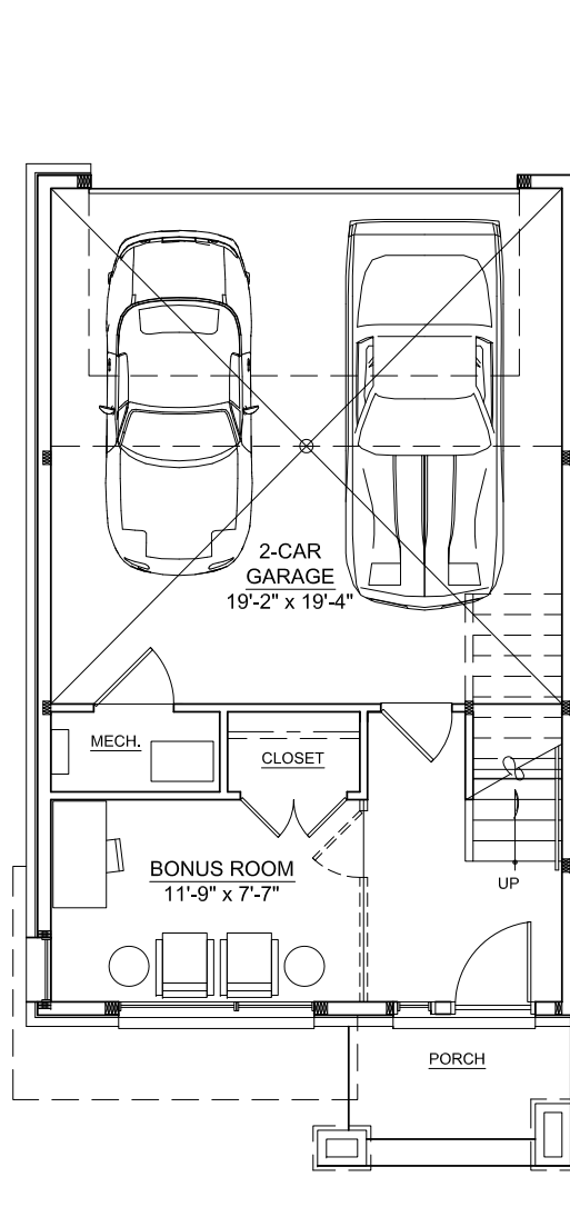
FIRST FLOOR PLAN 247 G.S.F. 0 1 2 4 6 8 FT.
