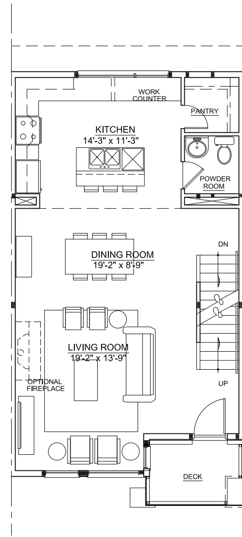
SECOND FLOOR PLAN 671 G.S.F. 0 1 2 4 6 8 FT.
