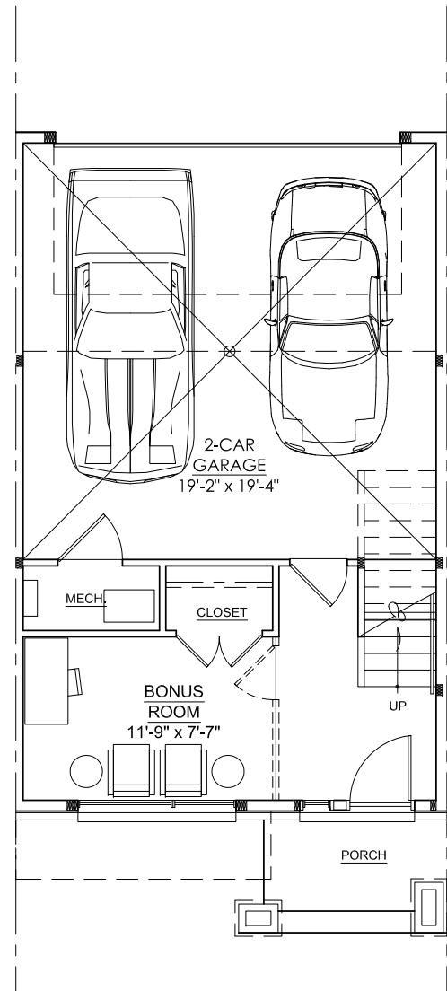
FIRST FLOOR PLAN 242 G.S.F. 0 1 2 4 6 8 FT.
